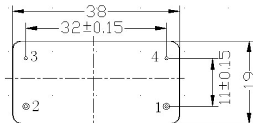
Bottom View Unit: mm
